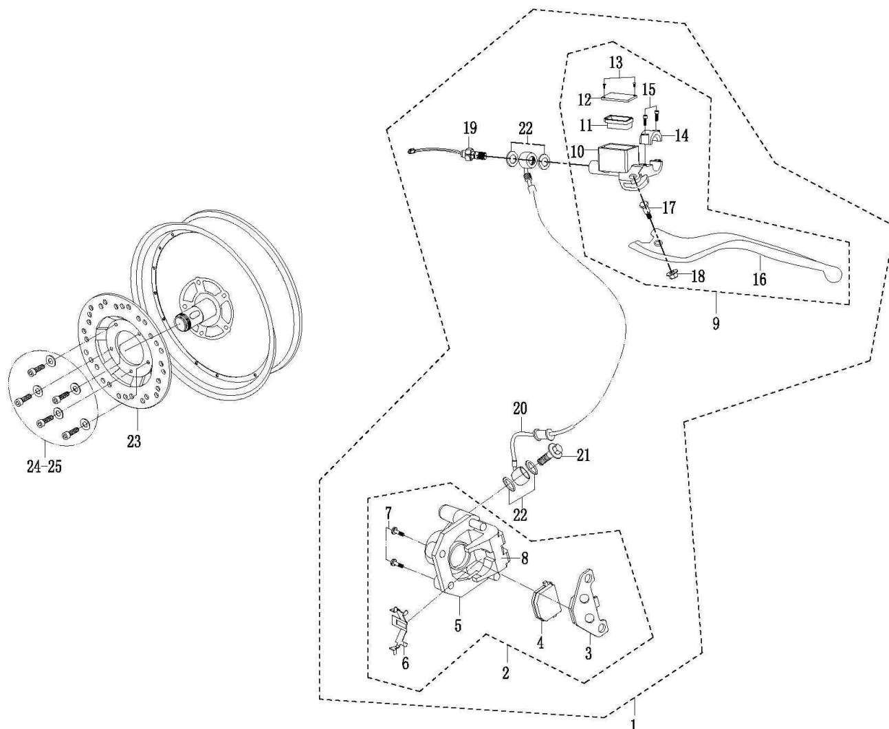
8-Rear brake system
