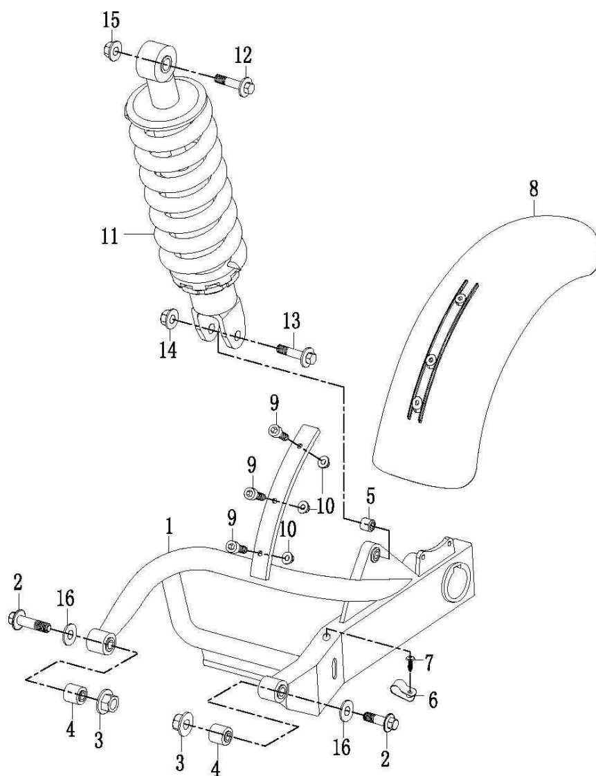
4-Rear suspension
