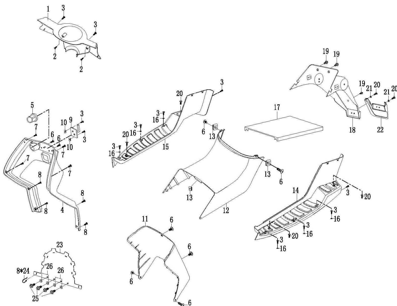
12-Black cover
