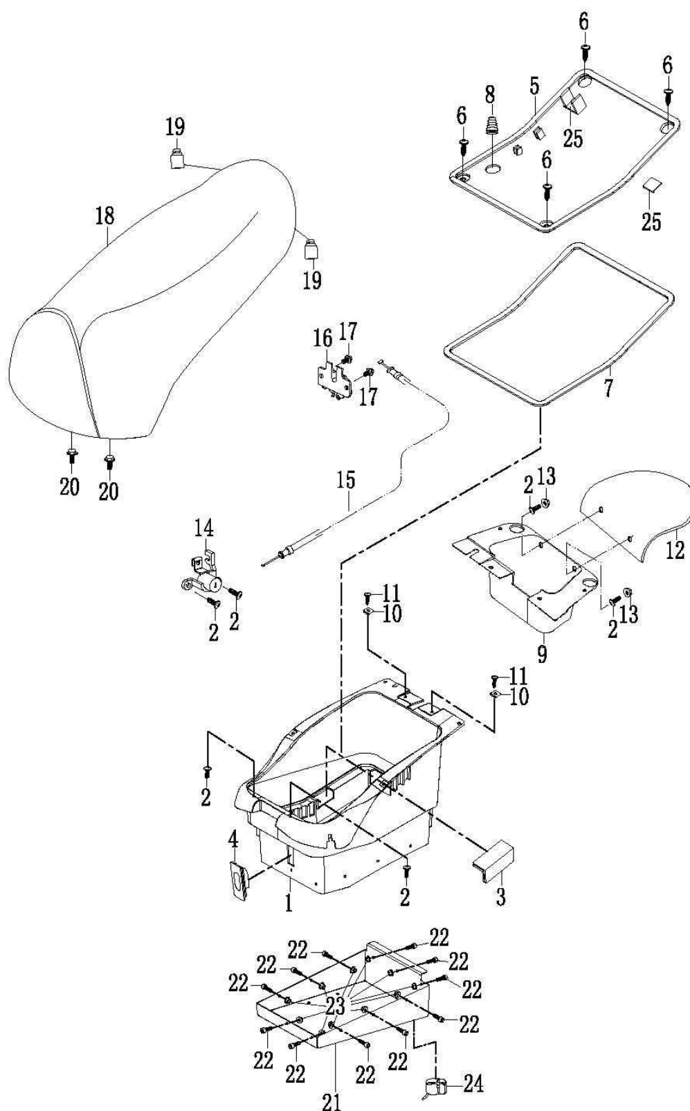
14-Seat/seat box
