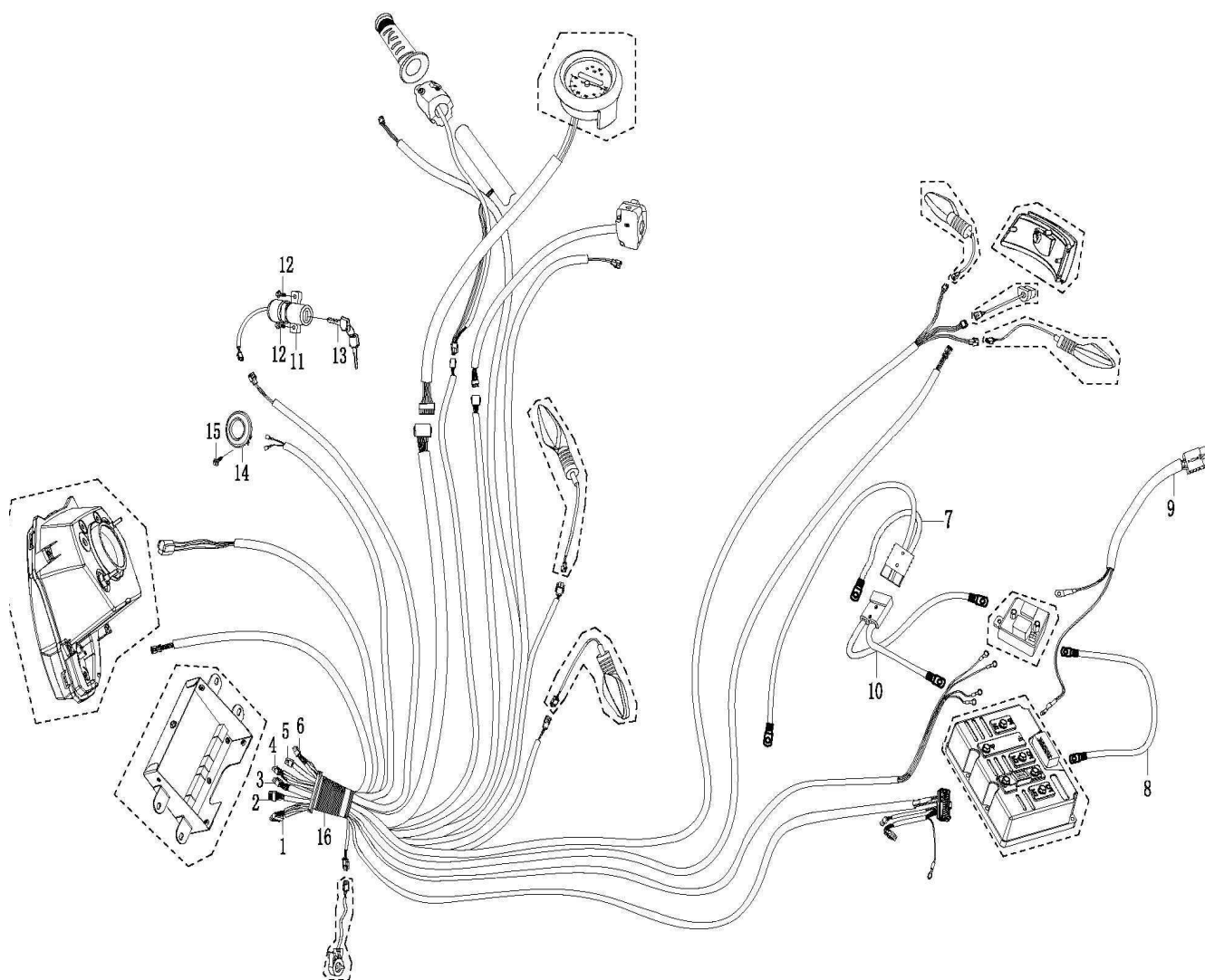
19 - Electric wire harness.
