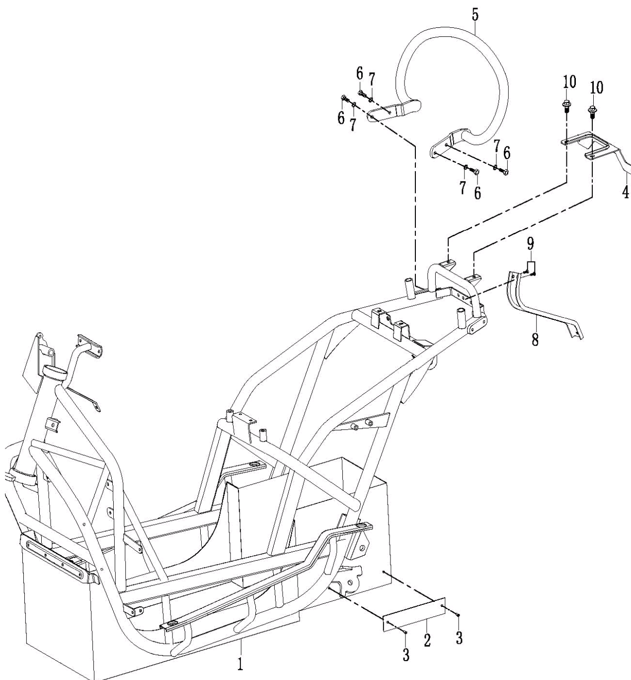
1-Frame main
