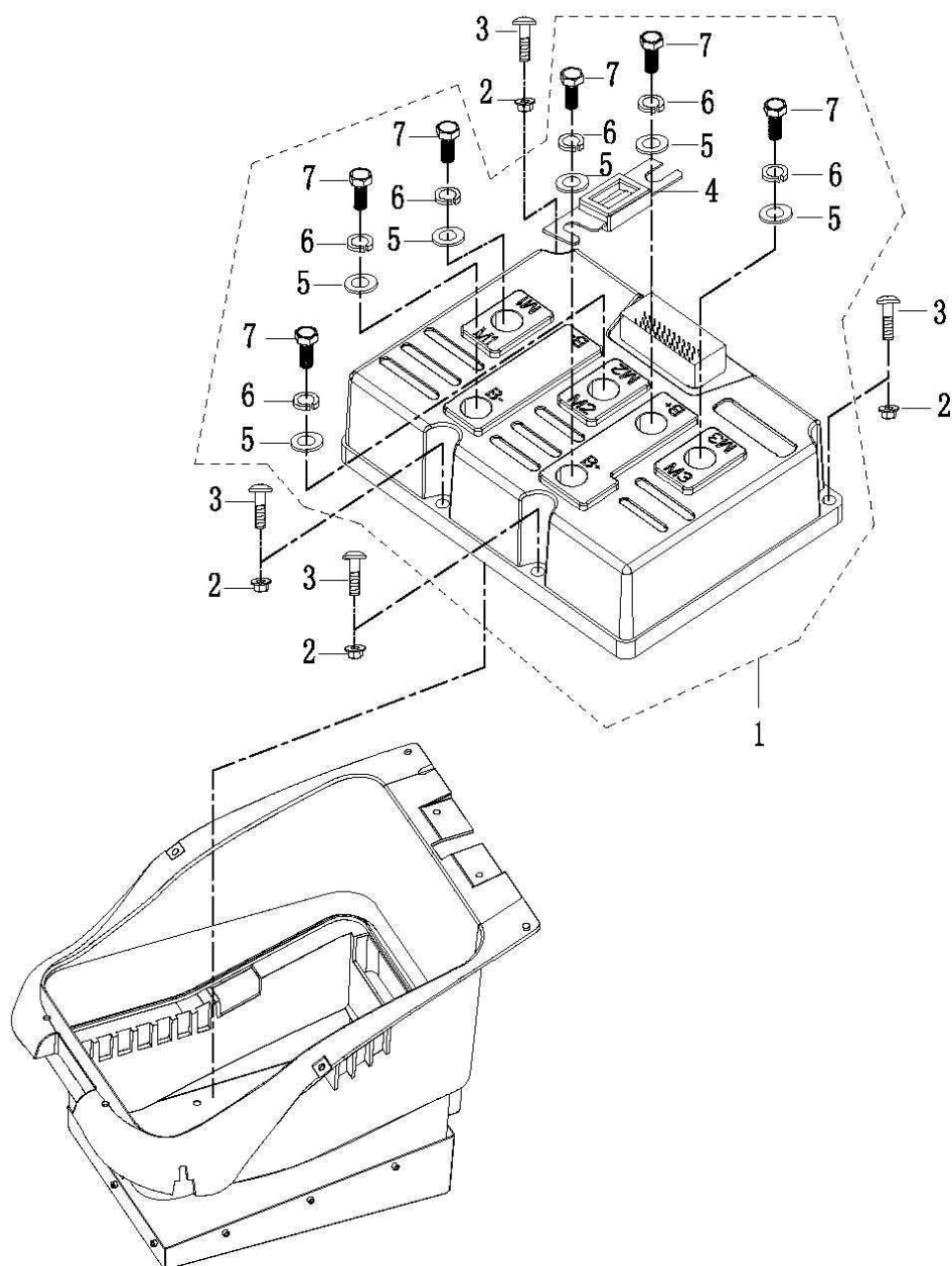
15-converter
